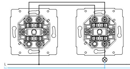
switch arrangement 6 stair switch (change-over switch), singlepole 2-way switch without switched off position
