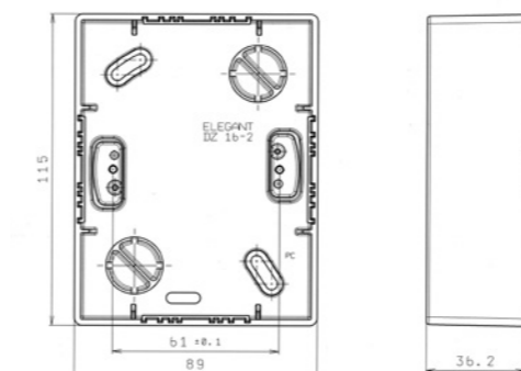
double outlet installation box, on-plaster
