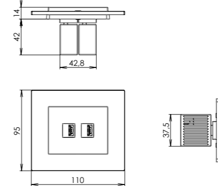
modular outlet USB with charger
