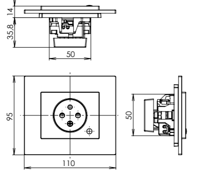
single outlet with safety shutters and overvoltage protection (light indication)
