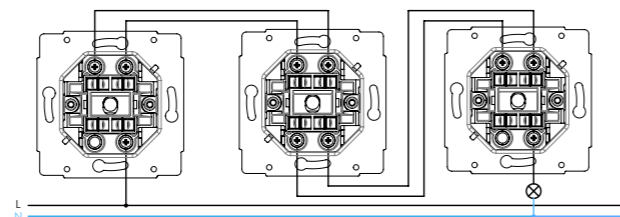
switch arrangement 6+7+6 change-over switch - cross-bar switch - change-over switch
