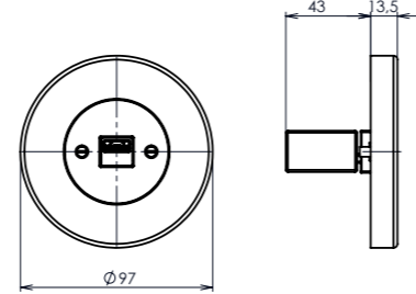
outlet with USB charging
