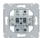
fitting, arrangement 5 serial change-over switch 10 AX, 250 V AC
