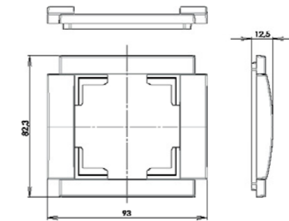
double frame horizontal
