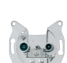
TV+R outlet through, branching attenuation 9 dB for coaxial cables of diameter 4.5–8.3 mm type designation on the product: ZAP9/K
