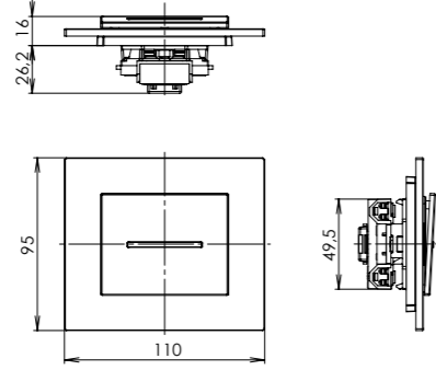
switch with single cover with backlighting
