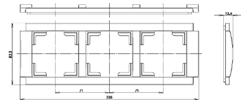
triple frame horizontal
