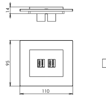
modular data outlet HDMI, USB, RJ45
