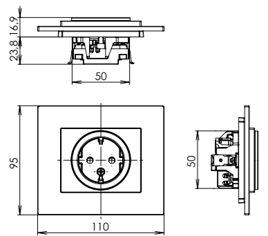
schuko single outlet with safety shutters
