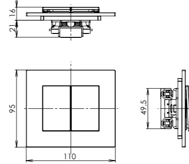
switch with double cover
