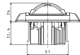
motion sensor STEINEL
