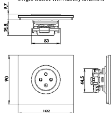
single outlet with safety shutters
