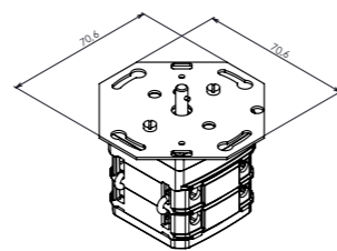
two level cam switch
