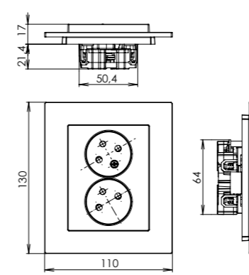
double outlet with safety shutters
