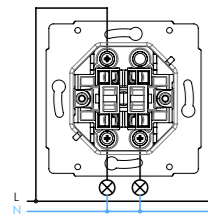
switch arrangement 5 (serial change-over switch, singlepole) two circuit switch with switched-off position)
