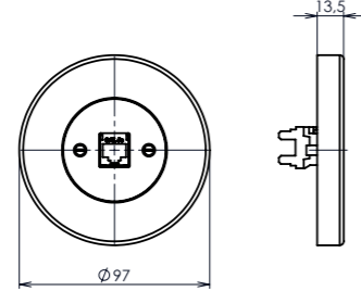
outlet with connector PC, RJ 45
