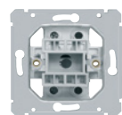
fitting, arrangement in singlepole switch with a zero terminal 10 AX, 250 V AC
