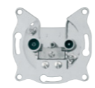
TV+R outlet terminal, attenuation 1 dB, 350 mA, 24 V DC for coaxial cables of diameter 4.5–8.3 mm type designation on the product: ZAR 1/K
