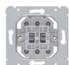
fitting, arrangement 6/0+6/0 shutter switch with locking 10 AX, 250 V AC
