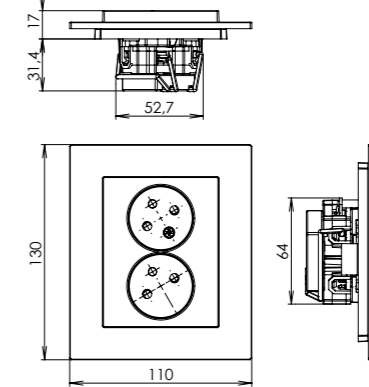
double outlet with safety shutters and overvoltage protection (audible alarm or light indication)
