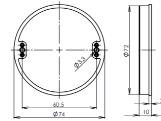
spacer ring VK1
