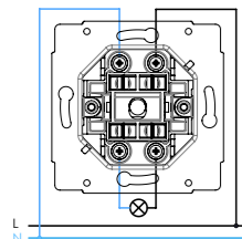
switch arrangement 2 (twopole switch)
