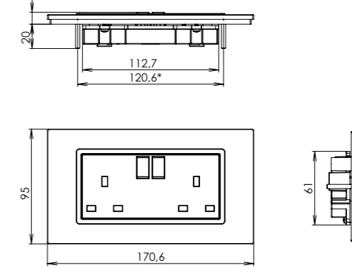
double outlet British standard
