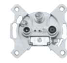
TV+R+SAT outlet through, attenuation 10 dB, 300 mA, 24 V DC for coaxial cables of diameter 4.5–8.3 mm type designation on the product: ZAR-SAT 10/P3
