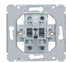
fitting, arrangement 1/0+1 switching controller + singlepole switch 10 AX, 250 V AC
