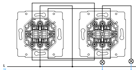
switch arrangement 6+6 double stair switch (serial change-over switch)
