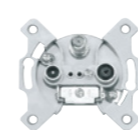
TV+R+SAT outlet terminal, attenuation 1 dB, 300 mA, 24 V DC for coaxial cables of diameter 4.5–8.3 mm type designation on the product: ZAR-SAT 1.4/K
