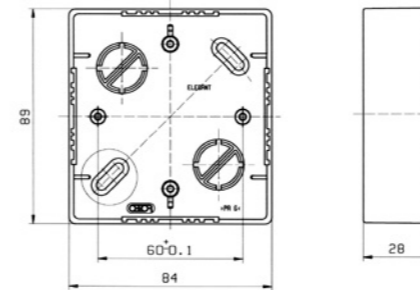
installation box, on-plaster
