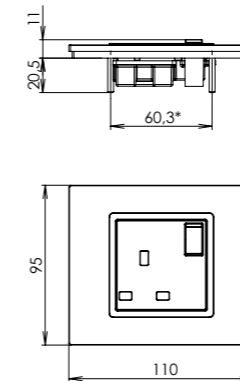
single outlet British standard
