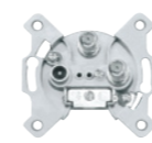
TV+SAT+SAT outlet through, attenuation 10 dB, 300 mA, 24 V DC for coaxial cables of diameter 4.5–8.3 mm type designation on the product: ZAR-SAT 10/P3
