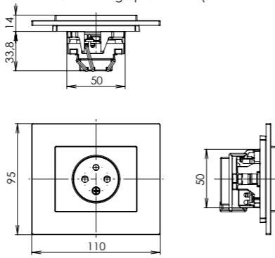
single outlet with safety shutters and overvoltage protection (audible alarm)
