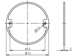
spacer ring VK2
