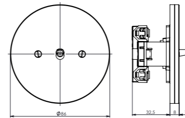
house switch with frame arrangement 1, 2, 6, 7, 1/0
