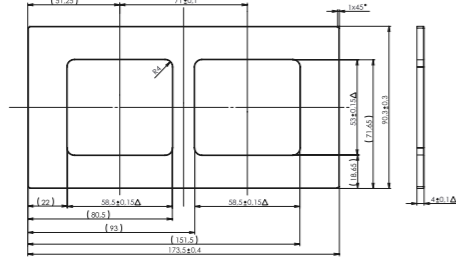
double frame horizontal
