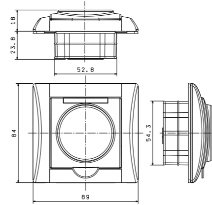
IP 44 single sockets with a lid and safety shutters
