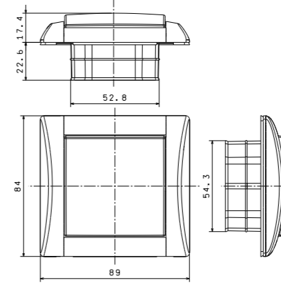
IP 44 switch with single cover
