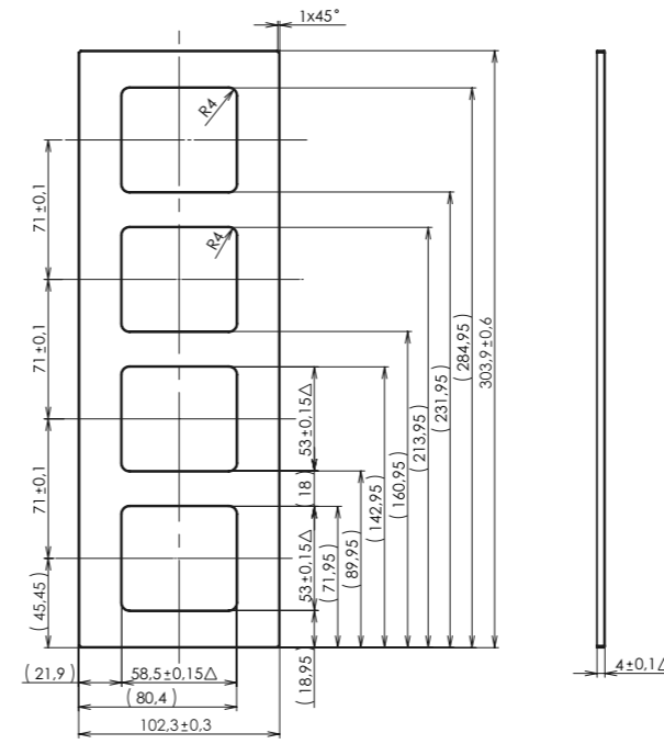
fourfold frame vertical
