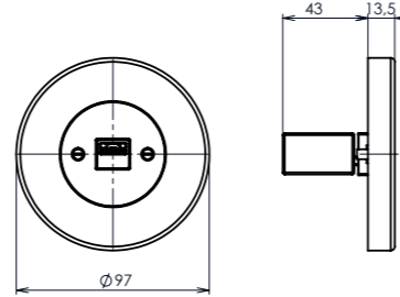
sockets with USB-A charging
