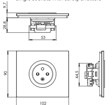
single sockets with safety shutters
