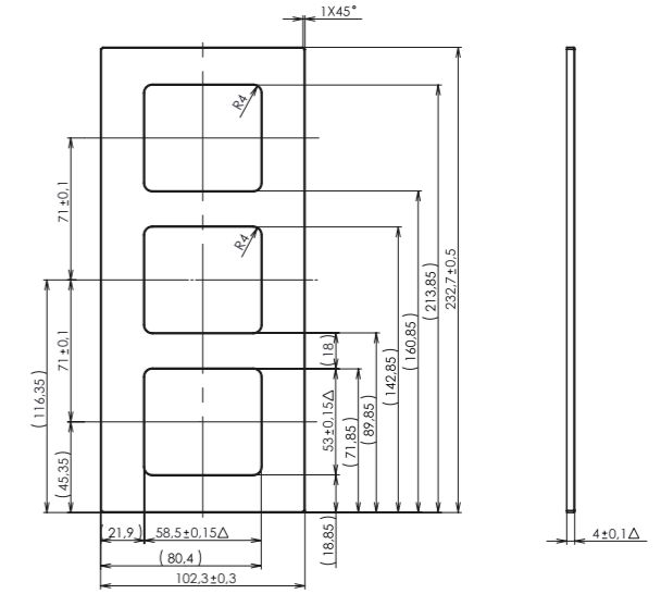
triple frame vertical
