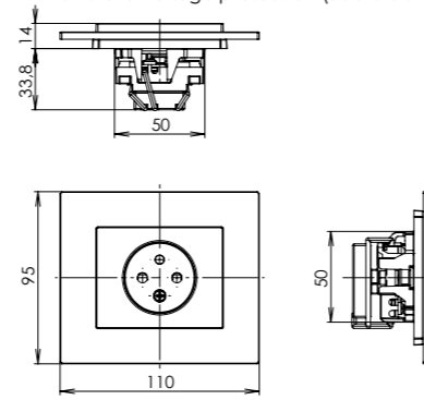
single sockets with safety shutters and overvoltage protection (audible alarm)
