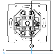
switch arrangement 1 (singlepole switch)
