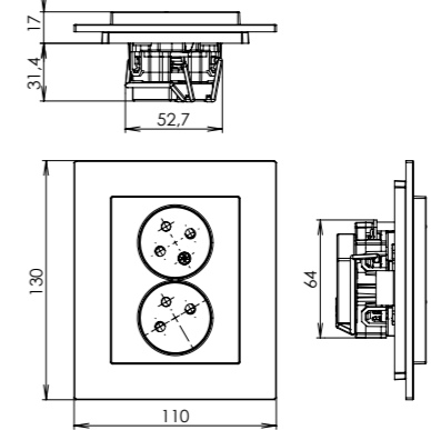
double sockets with safety shutters and overvoltage protection (audible alarm or light indication)
