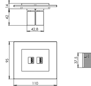
modular sockets USB with charger
