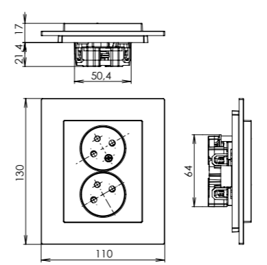
double sockets with safety shutters
