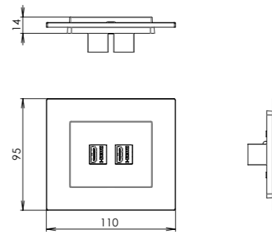
modular data sockets HDMI, USB, RJ45
