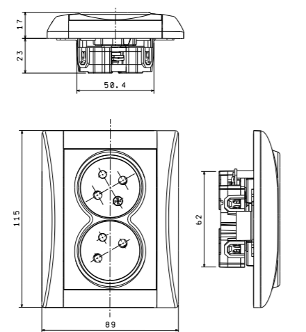
double sockets with/without safety shutters
