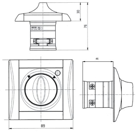
shutter controller
