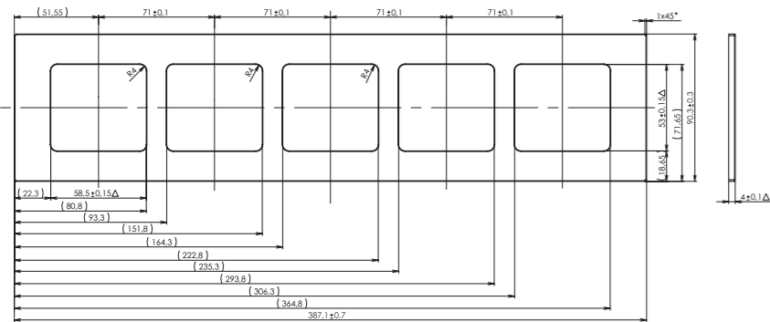
fivefold frame horizontal
