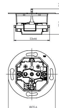
schuko single sockets
