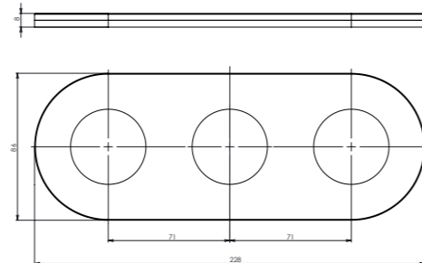
triple frame horizontal and vertical
