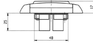
communication sockets
