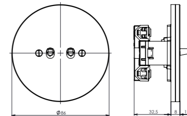
house switch with frame arrangement 5, 6+6, 6/0+6/0
