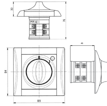
rotary cooker switch
