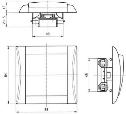
switch with single cover
