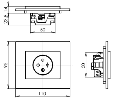
single sockets with safety shutters
