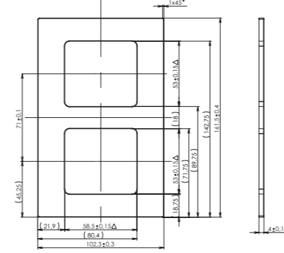
double frame vertical
