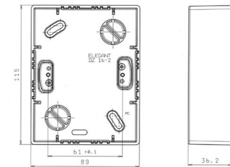
double sockets installation box, on-plaster
