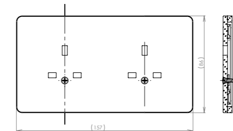
double socket british standard
