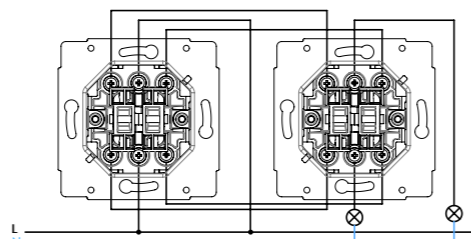
switch arrangement 6+6 double stair switch (serial change-over switch)
