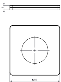
single frame
