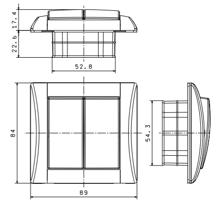
IP 44 switch with double cover
