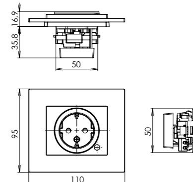
single sockets with safety shutters and overvoltage protection (light indication and audible alarm)
