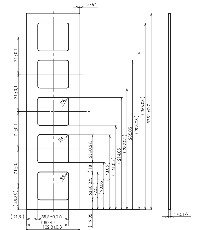
fivefold frame vertical
