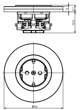
schuko single sockets with frame
