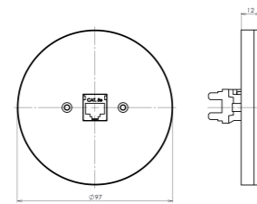
PC, RJ 45 sockets glass
