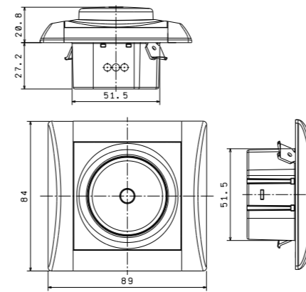
PUSH-PULL rotary dimmer switch
