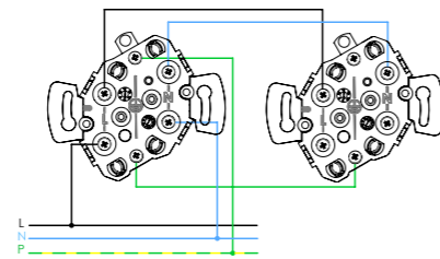
double sockets
