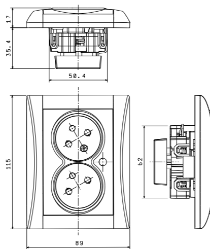
double sockets with overvoltage protection
