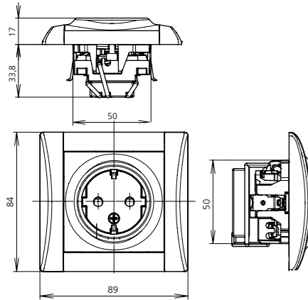
single schuko sockets with overvoltage protection (audible alarm)
