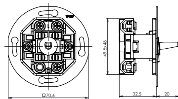
house switch arrangement 1, 2, 5, 6
