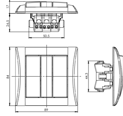
switch with triple cover
