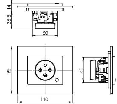
single sockets with safety shutters and overvoltage protection (light indication)
