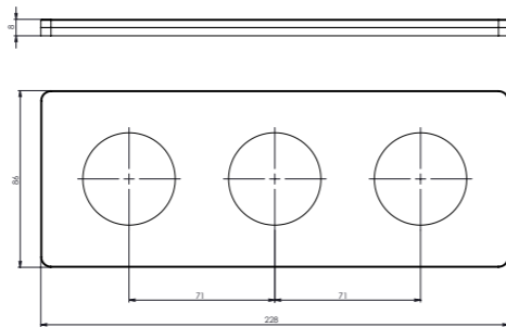
triple frame horizontal and vertical
