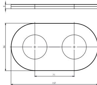
double frame horizontal and vertical
