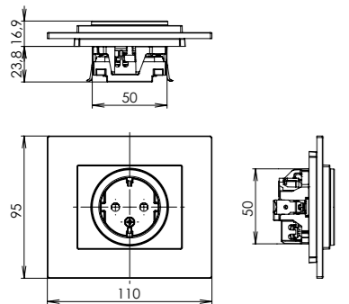
schuko single sockets with safety shutters
