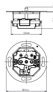
single sockets
